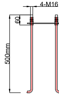
ANCHOR BOLT DETAIL
