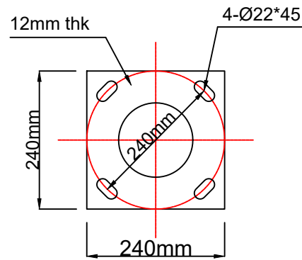
BASE PLATE
