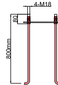
ANCHOR BOLT DETAIL
