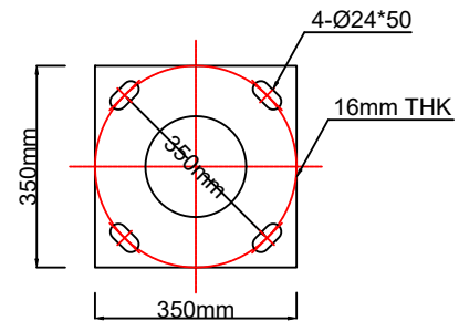
BASE PLATE
