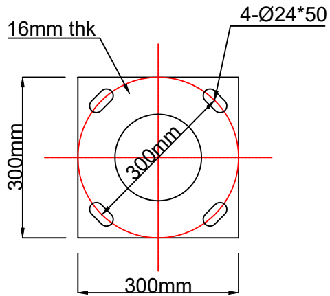
BASE PLATE
