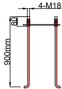
ANCHOR BOLT DETAIL
