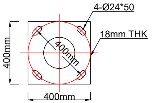
BASE PLATE
